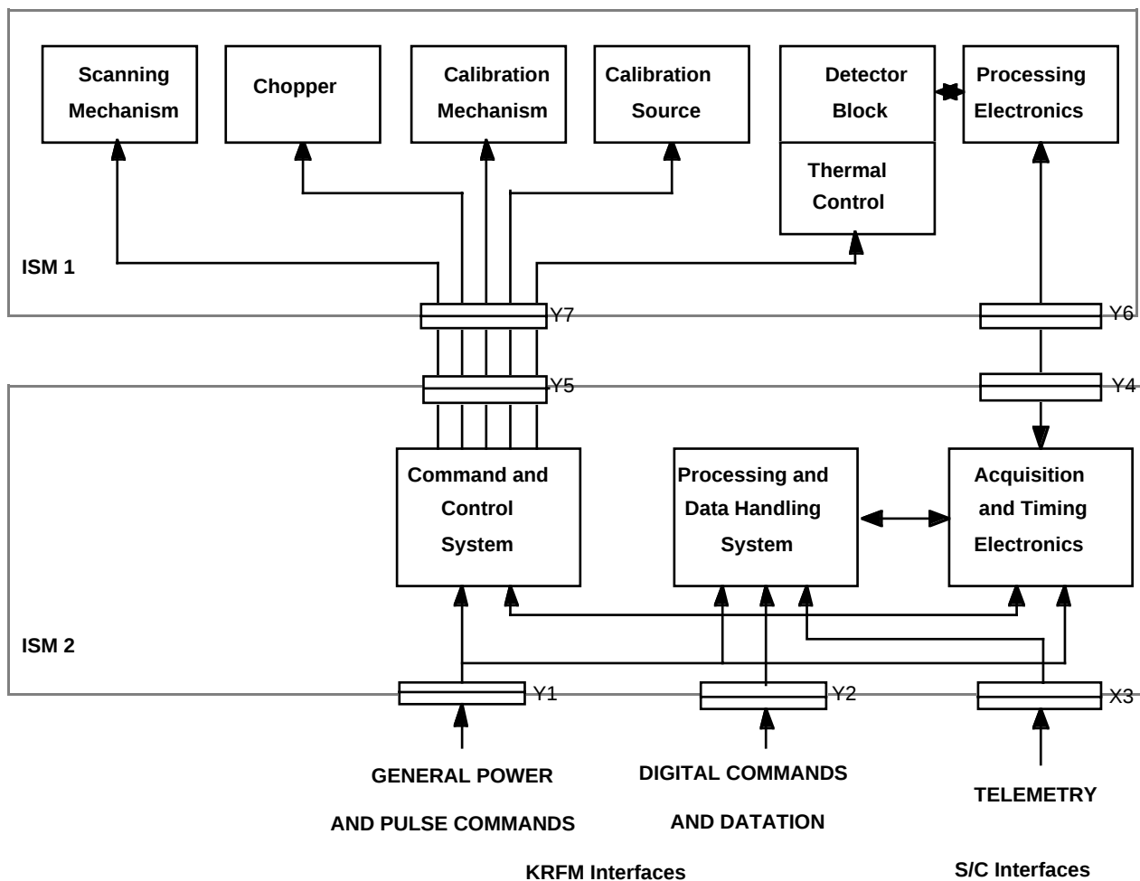
Figure 2: Electronic Bloc-diagram
