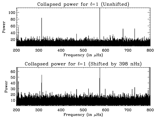
Figure 5. Collapsed power for l = 1 and m = 0, \pm 1 not shifted (top) and collapsed power for the same three modes shifted by m \times 398 nHz, a reasonable core rotation rate. This is for SOI/MDI velocity in a range where p_1 - p_4 would be. The high peaks are artefacts from the spacecraft modulation and the ‘multiplet’ structure in the lower collapsogram identifies them as such.
