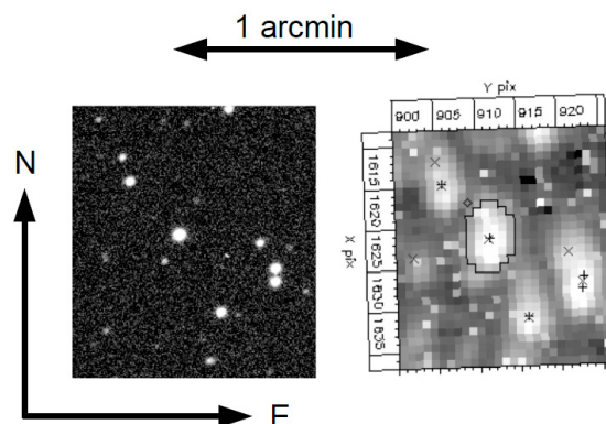
Fig. 2. The sky area around CoRoT-12 (brightest star near the centre). Left: R-filter image with a resolution of 1.3'' taken with the INT/WFC. Right: image taken by CoRoT, at the same scale and orientation. The jagged outline in its center is the photometric aperture mask; indicated are also CoRoT's x and y image coordinates and positions of nearby stars from the Exo-Dat (Deleuil et al. 2009) database.
