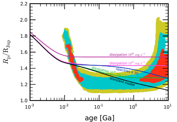
Fig. 8. Evolution of the size of CoRoT-12b (in Jupiter units, R_{\text{Jup}} ) as a function of age (in billion years), compared to constraints inferred from CoRoT photometry, spectroscopy, radial velocimetry and CESAM stellar evolution models. Red, blue and yellow-green dots correspond to the planetary radii and ages that result from stellar evolution models matching the inferred \rho_*\text{-}T_{\text{eff}} uncertainty ellipse within 1\sigma , 2\sigma and 3\sigma , respectively. Planetary evolution models for a planet with a solar-composition envelope and no core are shown as plain lines and are labeled as follow: standard (black): irradiated planet with no extra heat source; opacities \times 30 (blue): opacities have been artificially multiplied by 30 compared to standard model; dissipation : models in which 10^{26} (green), 10^{27} (pink), and 10^{28} (purple) \text{erg s}^{-1} is deposited at the planet’s center. These models assume a total mass of 0.92 M_{\text{Jup}} and an equilibrium temperature of 1450 K
