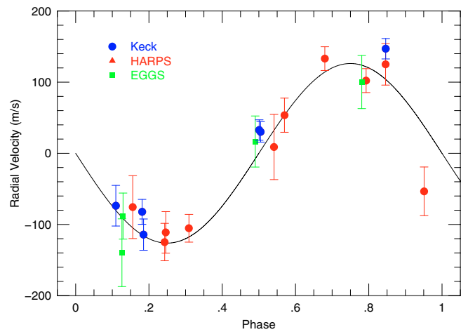
Fig. 3. HARPS and HIRES RVs phase-folded on the CoRoT ephemeris and overimposed on the best fit orbital model.
