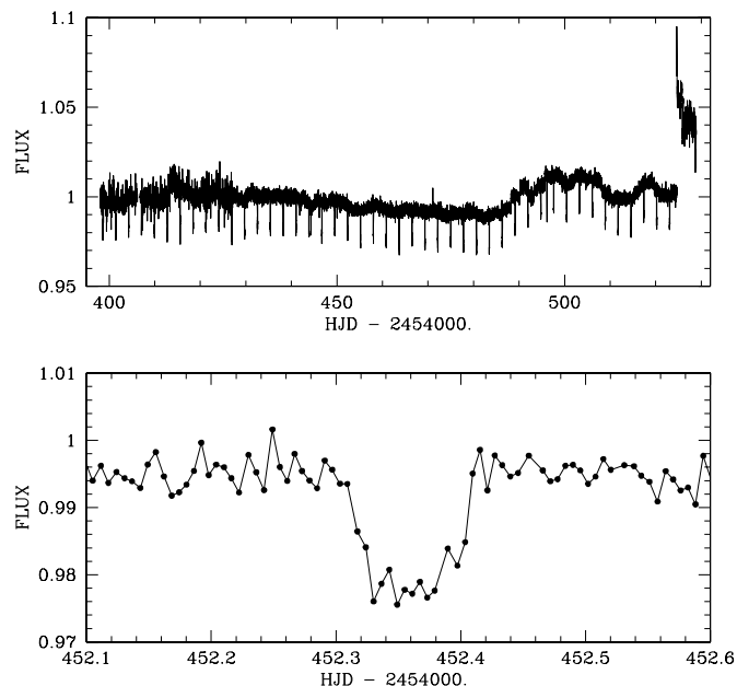
Fig. 1. Top: normalized CoRoT LC of the star CoRoT-12. The over-sampled part of the LC was binned to the same time bin than its first part for the sake of clarity. Bottom: zoom on a transit of CoRoT-12b.
