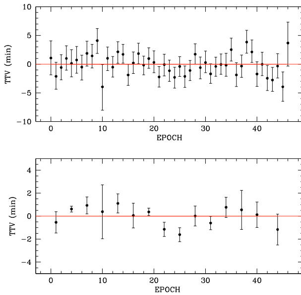
Fig. 6. Top: median value and 1\text{-}\sigma limits of the TTV posterior distributions obtained in MCMC_3 . Bottom: same curve obtained after binning the TTVs per three (error of each bin = error on the mean).
