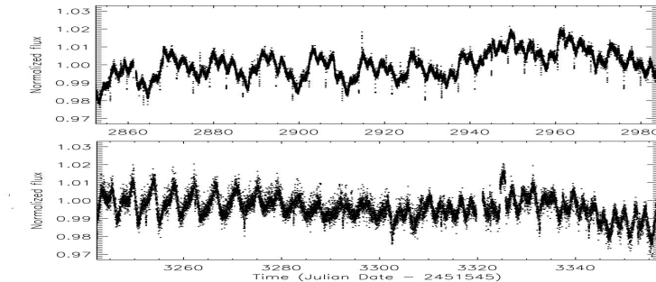
Figure 2.: Two examples of CoRoT light curves .
