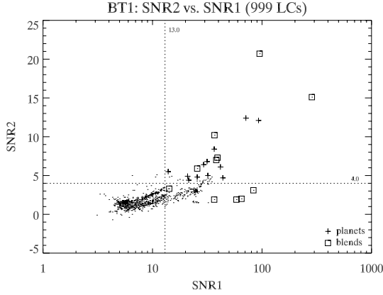
Figure 2. SNR_2 vs. SNR_1 diagram. Crosses and squares are overplotted on genuine planets and binary stars, respectively. A thresholding in SNR_2 selects all planets much more efficiently than a thresholding in SNR_1 .
