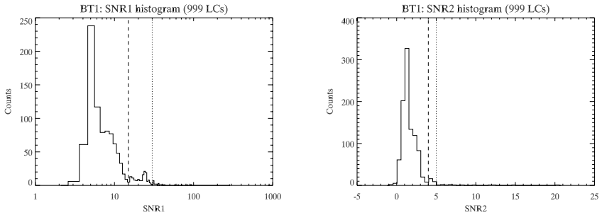
Figure 1. Left: SNR_1 histogram. The dashed and dotted lines mark thresholds at 15 and 30, respectively. Right: SNR_2 histogram. The dashed and dotted lines mark thresholds at 4 and 5, respectively.
