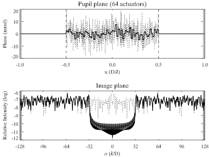
Figure 1. One-dimensional speckle nulling simulation. Top: Phase-aberrated wavefront (dotted line) and negative of DM shape (thick solid line). Bottom: Uncorrected coronagraphic image (dotted line), and corrected coronagraphic image with speckle field nulling (thin solid line) and with speckle energy minimization (thick solid line).
