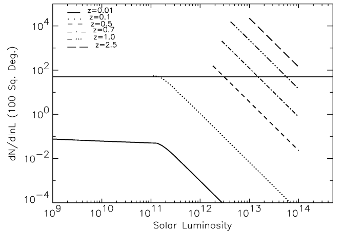
Figure 15. Number of starburst galaxies that can be detected in different redshift ranges (with a \Delta z/z = 0.5 ) at 350 \mu\text{m} by the confusion-limited survey of 100 deg 2 as a function of bolometric luminosity. The horizontal line shows the 50 sources needed in a \Delta z/z = 0.5 bin for \sim 14 per cent accuracy. The plots are limited to the fluxes above the detection limit and to luminosities below 10^{14} L_{\odot} .
